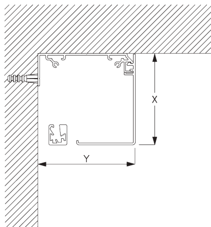
Fascia vierkant X = Fascia S 73 mm / Fascia L 110 mm Y = Fascia S 78 mm / Fascia L 110 mm
